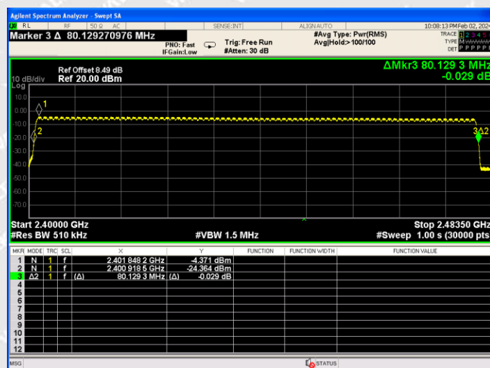
Hopping Sequence_2DH5
