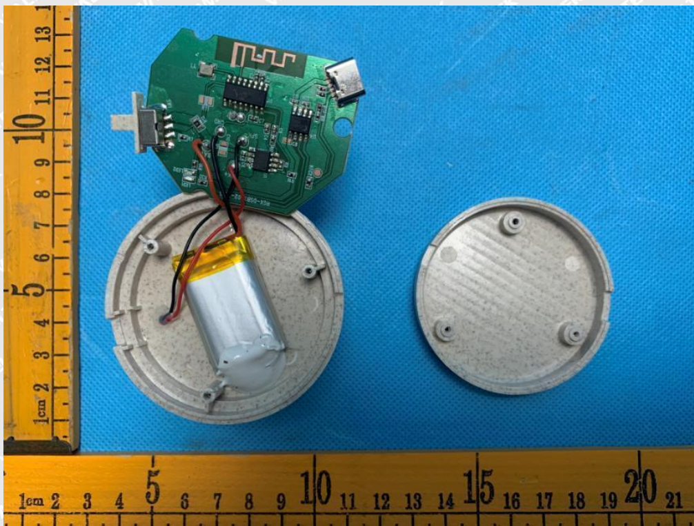
Photo 3 Internal view
