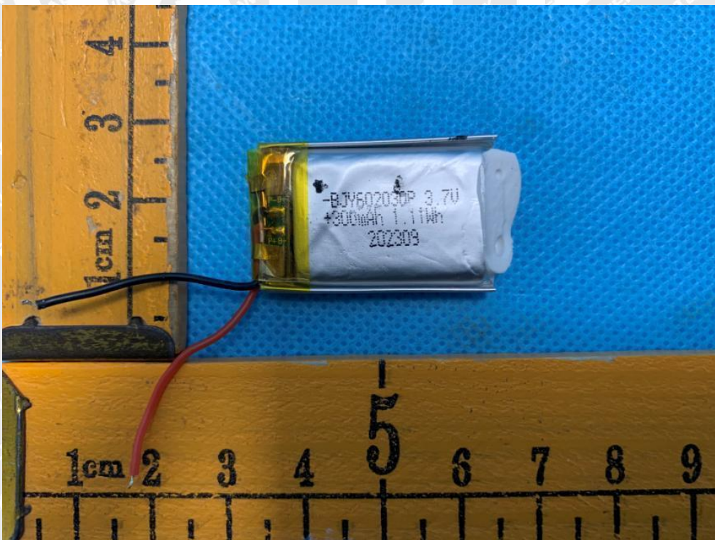
Photo 4 Battery view
