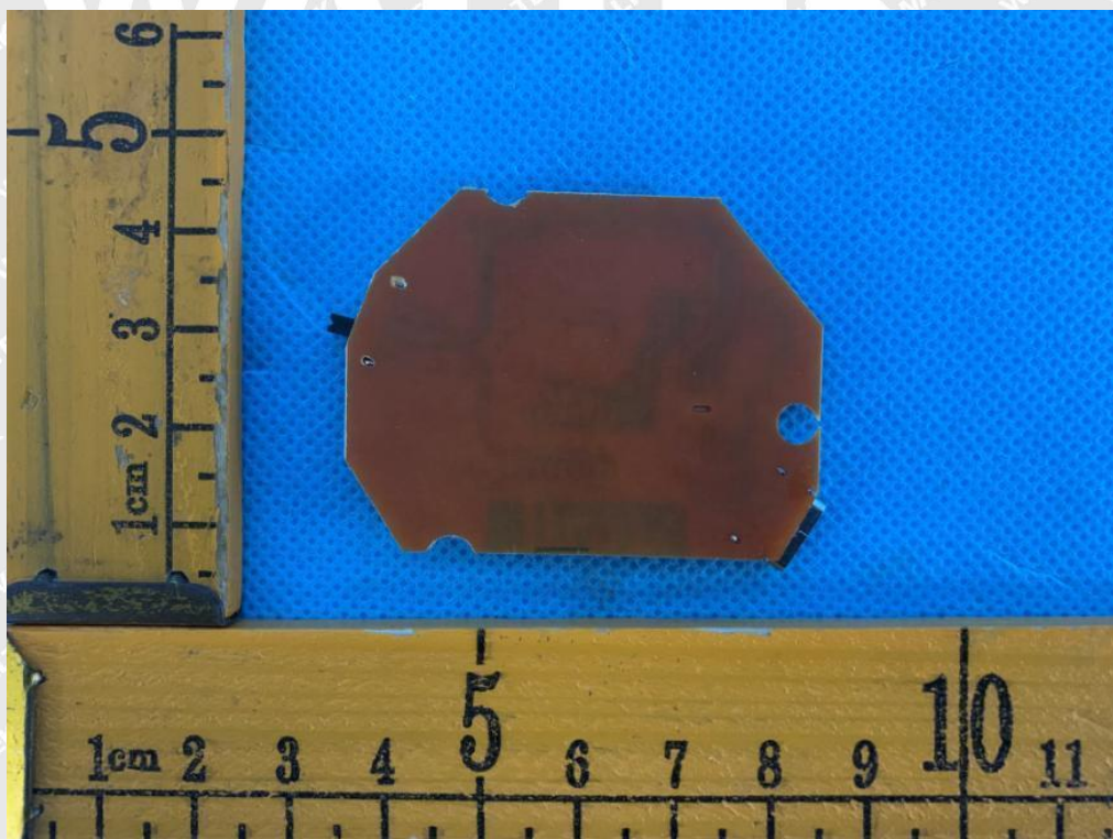
Photo 6 PCB view
