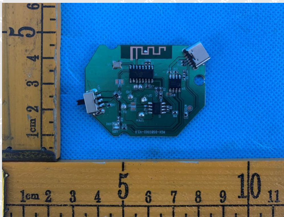
Photo 5 PCB view
