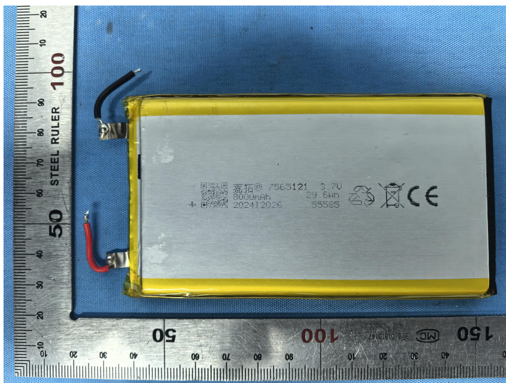
Fig. 11 –Battery view
