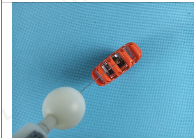
In the test, IP4X solid foreign matter contacts the metal wire
