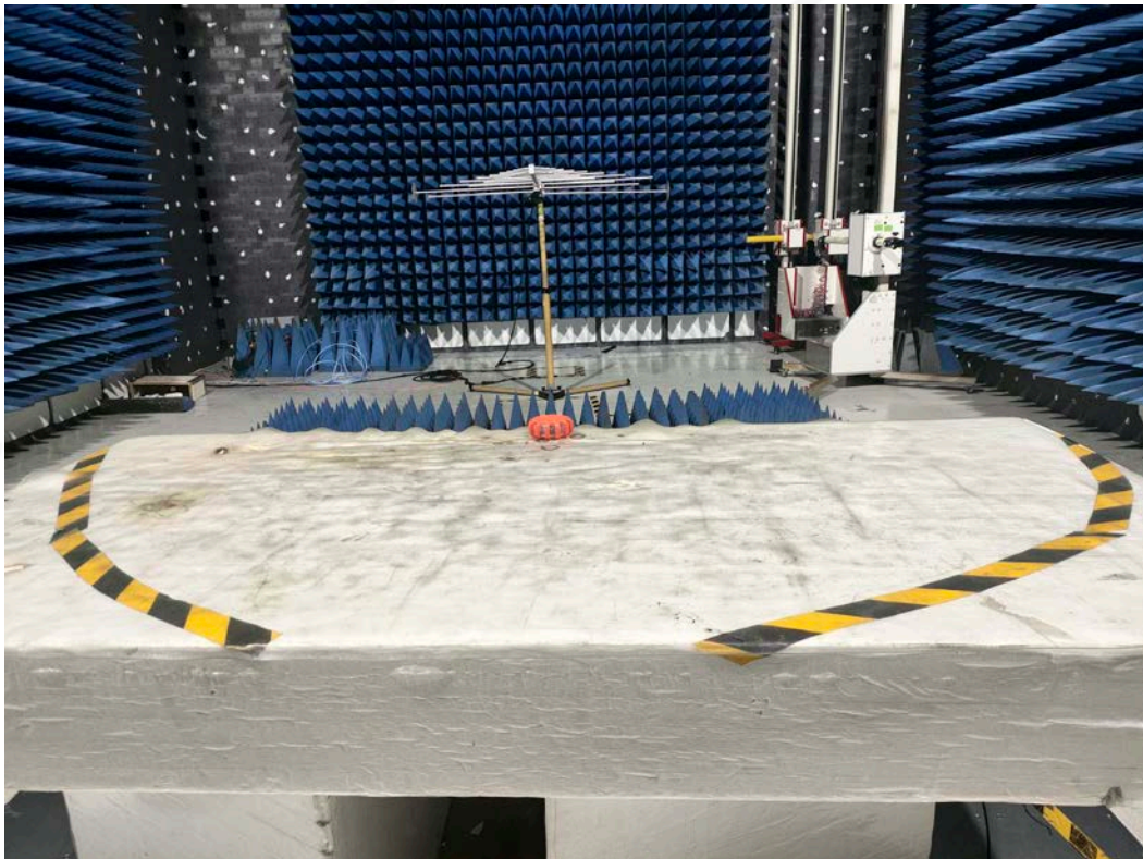
RS (80 - 1000 MHz)
