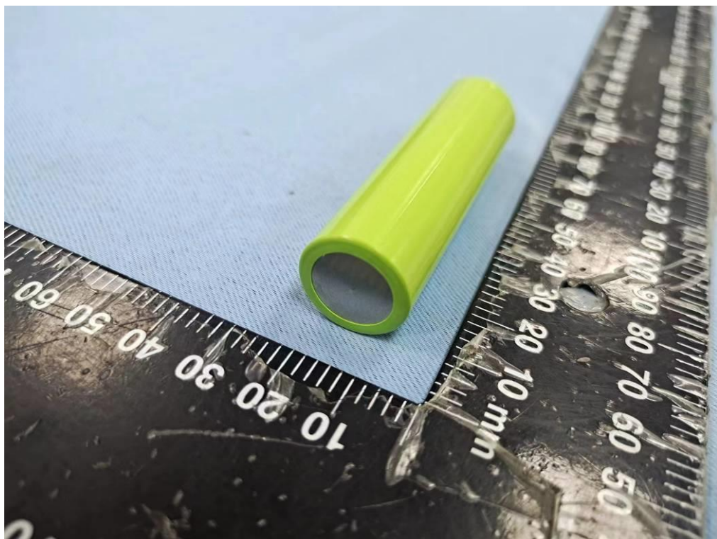
Picture 10 Bottom view of cell (Model: INR18650L26)
