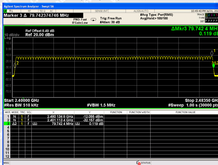
Hopping Sequence_DH5
