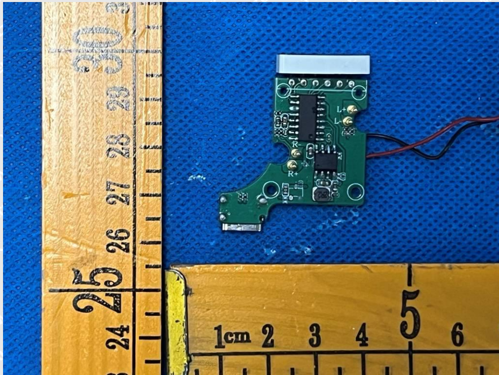
Figure 9: Internal view
