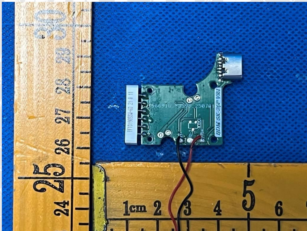
Figure 10: Internal view
