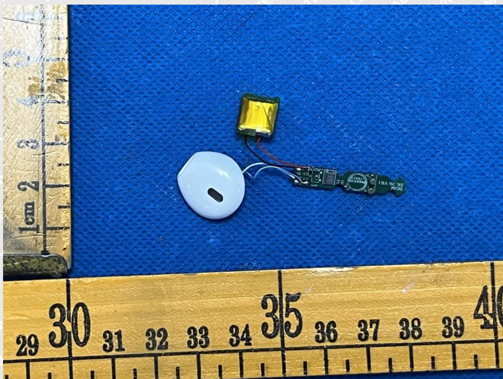
Figure 15: Internal view
