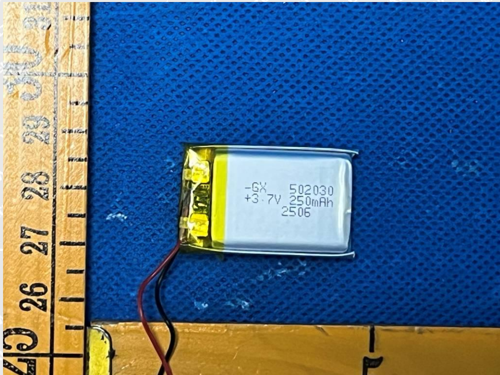
Figure 11: Battery for charging base
