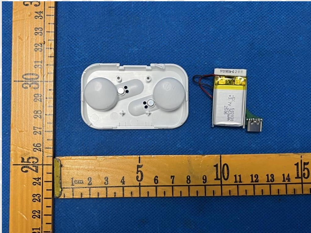
Figure 8: Internal view
