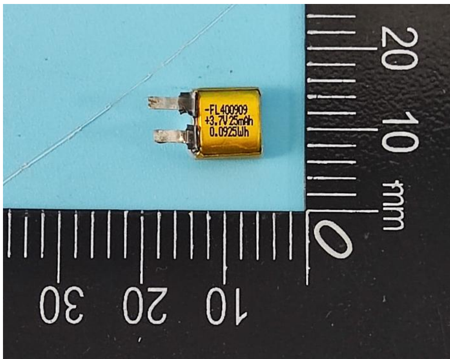
Photo 1 电池正面 Front view of Cell
