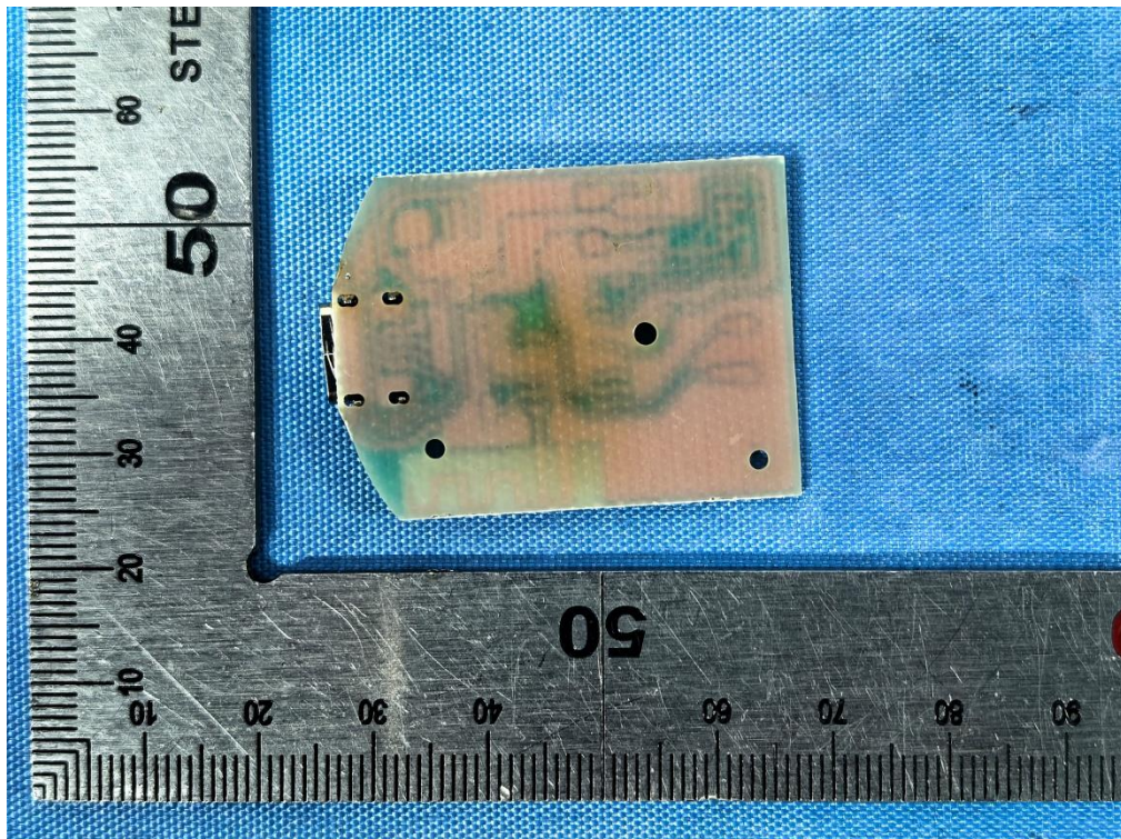
Fig.9 – PCB view
