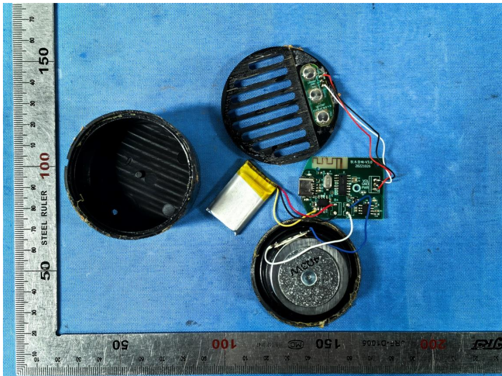
Fig.7 – open view
