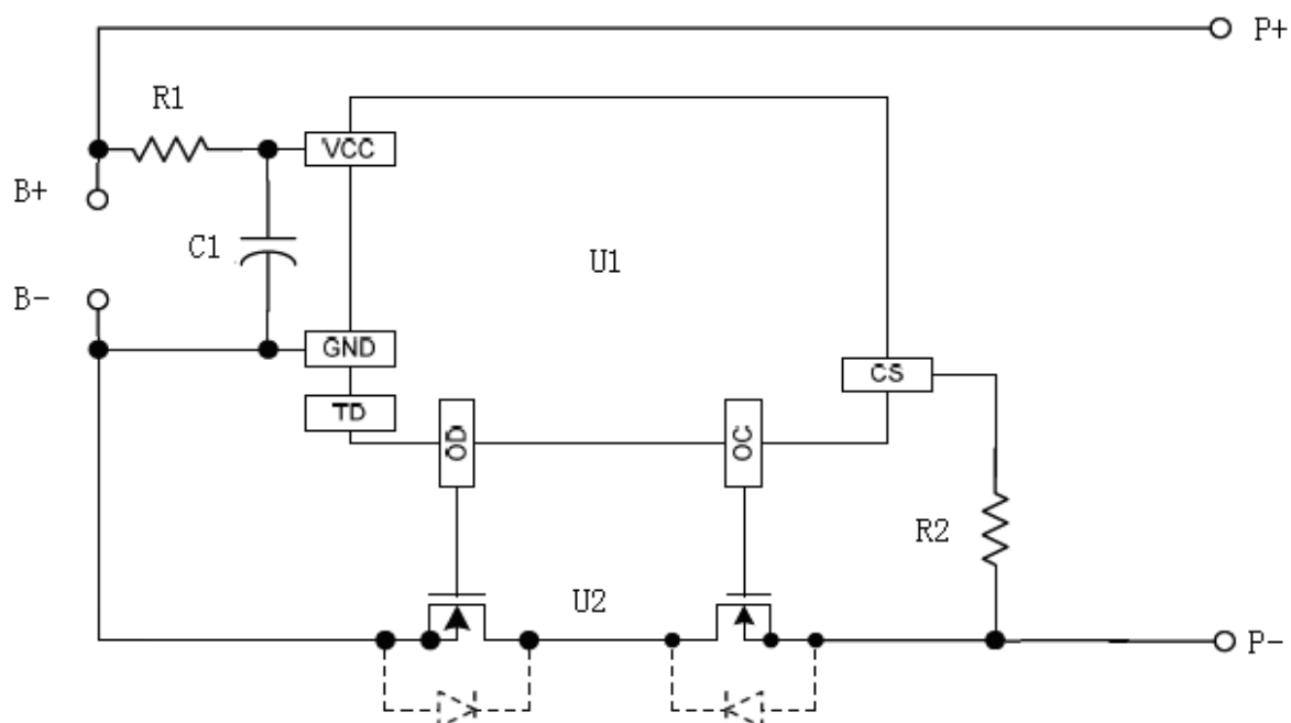
Circuit diagram:
