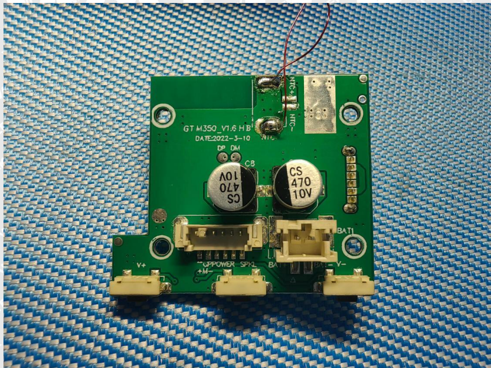
Figure 8: PCB view
