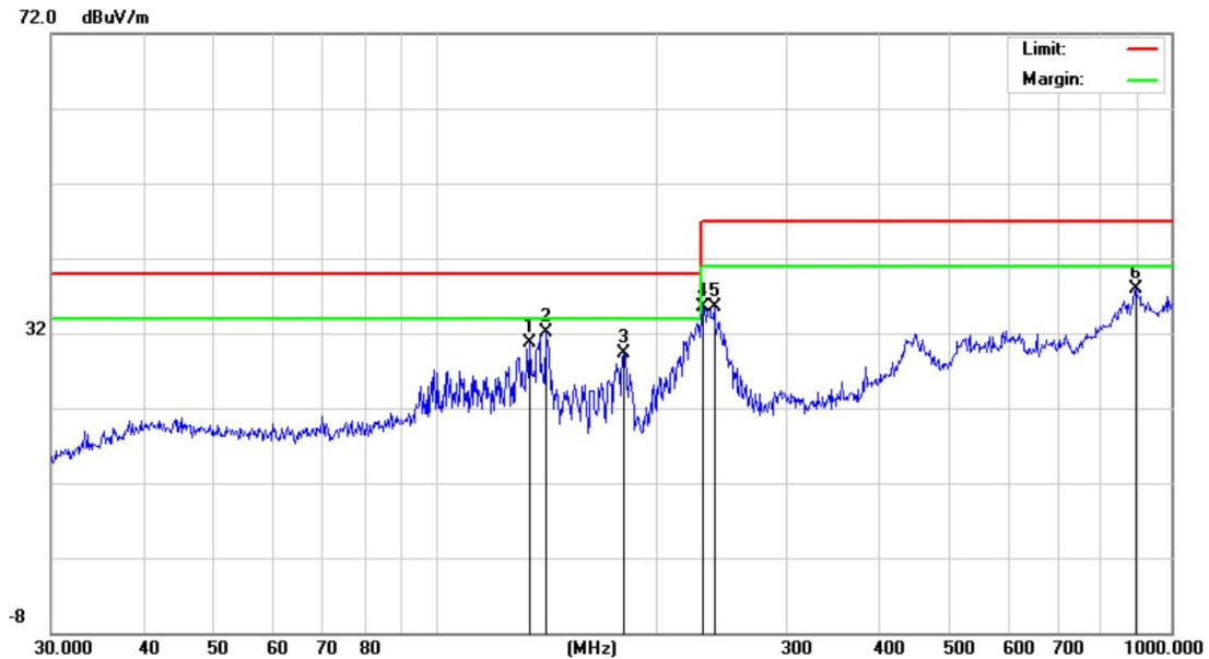
Test graph and data for Radiated Emission at Horizontal
