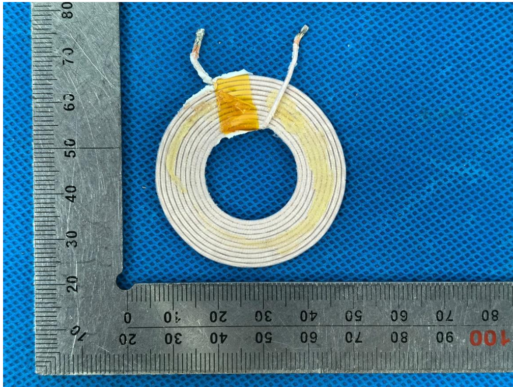
Fig.7 – Coil view
