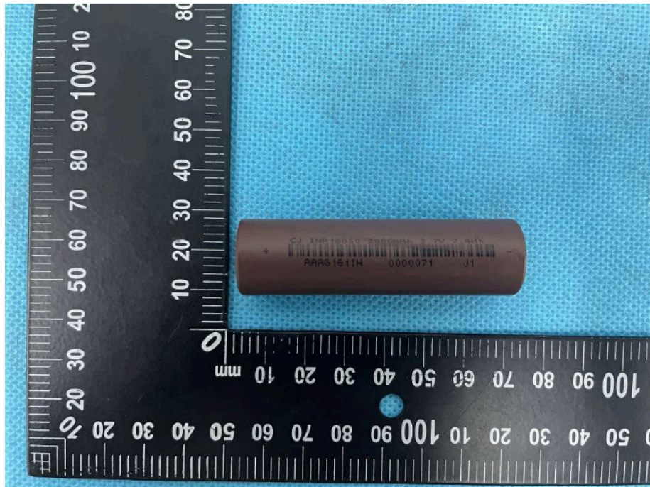
Figure 15 Front view of cell (Model: INR 18650-2000mAh)
