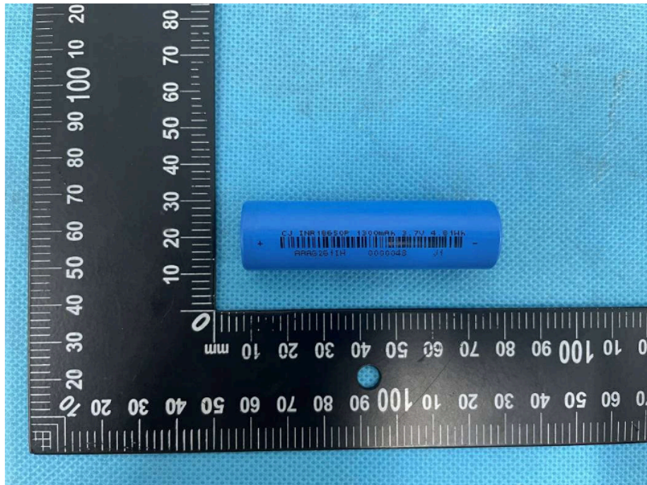
Figure 3 Front view of cell (Model: INR 18650P-1300mAh)
