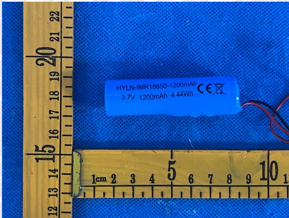
Figure 8: Battery view
