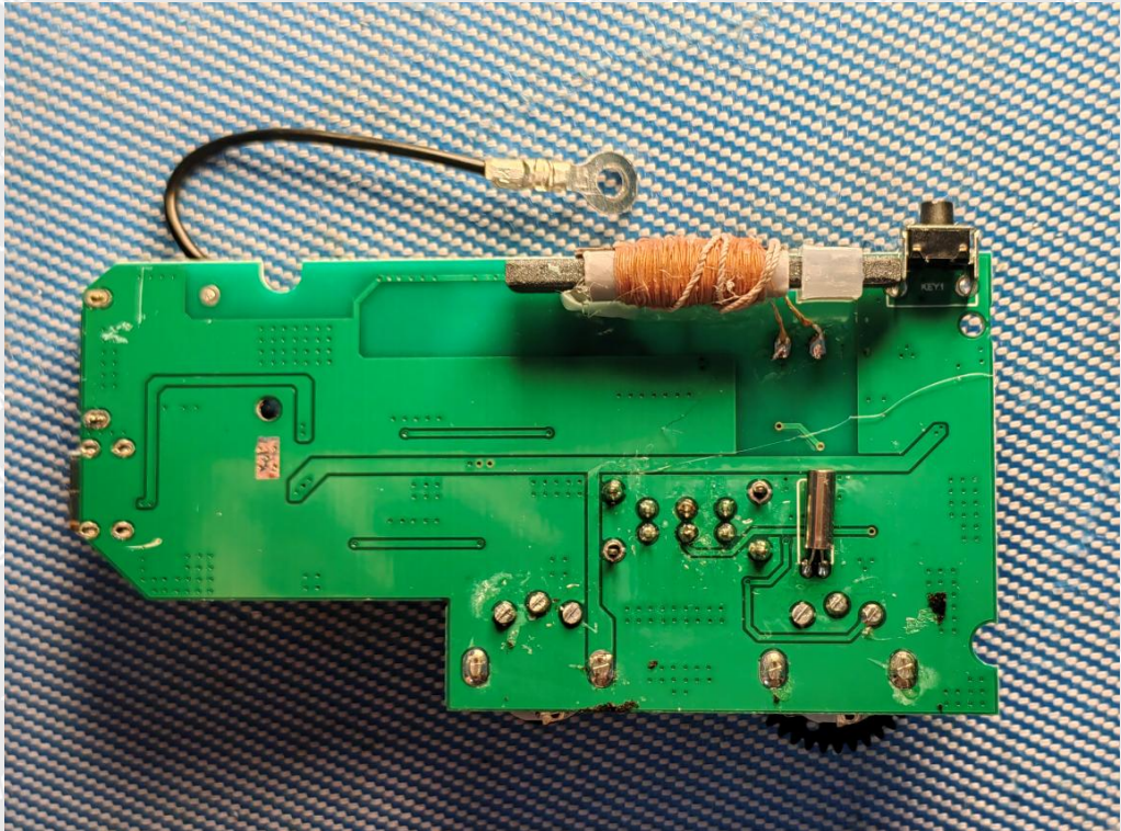
Figure 7: PCB view
