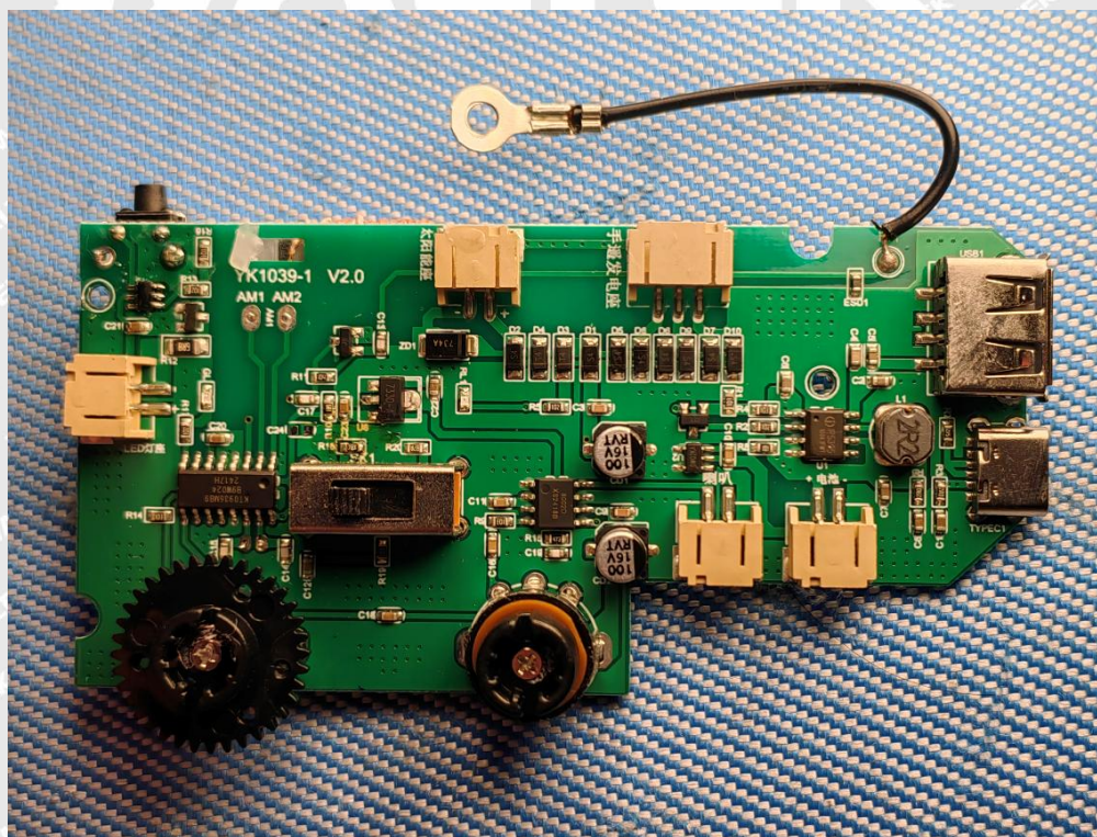
Figure 6: PCB view
