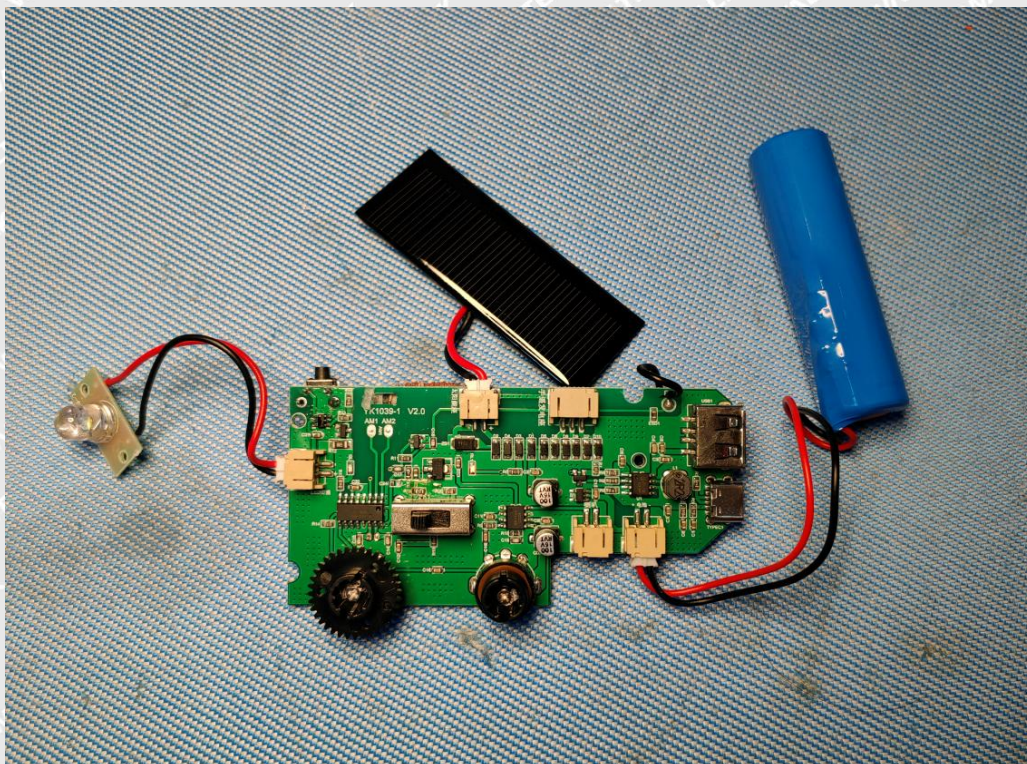
Figure 5: Internal view
