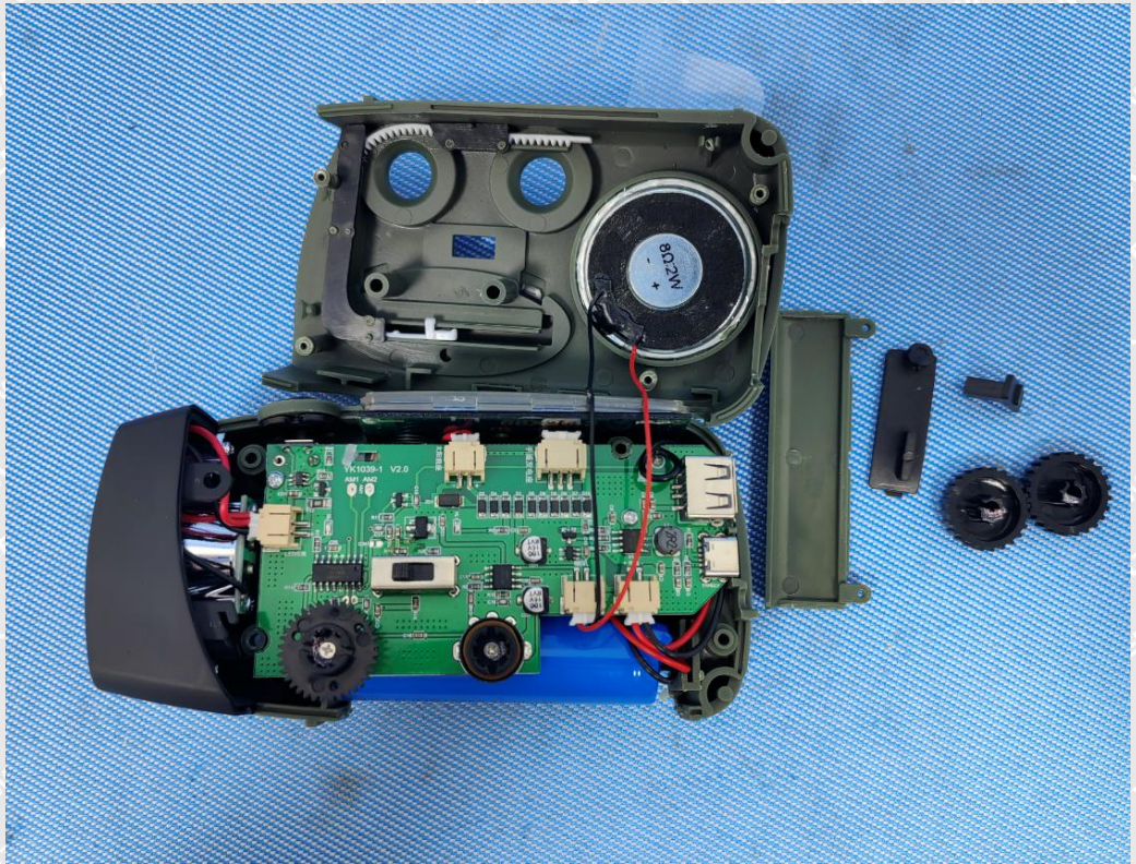
Figure 3: Internal view
