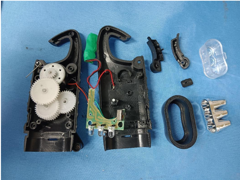
Fig.3– Uncover view of product
