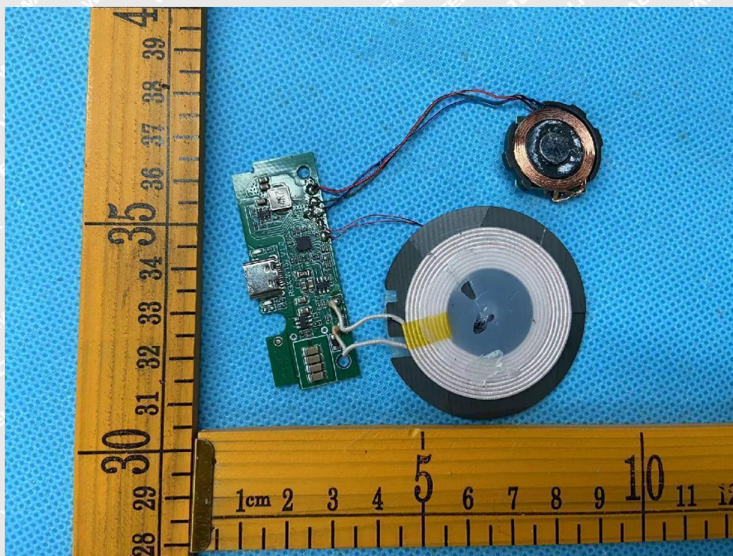
Figure 5 PCB view
