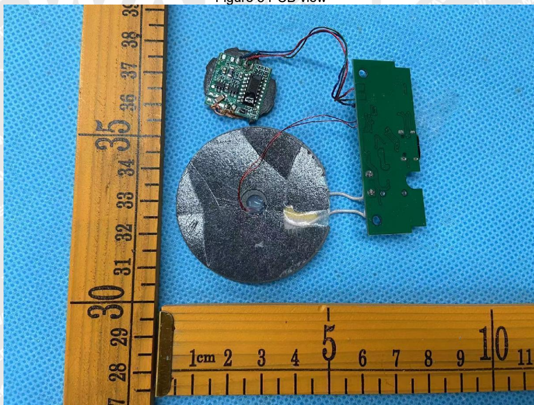
Figure 6 PCB view
