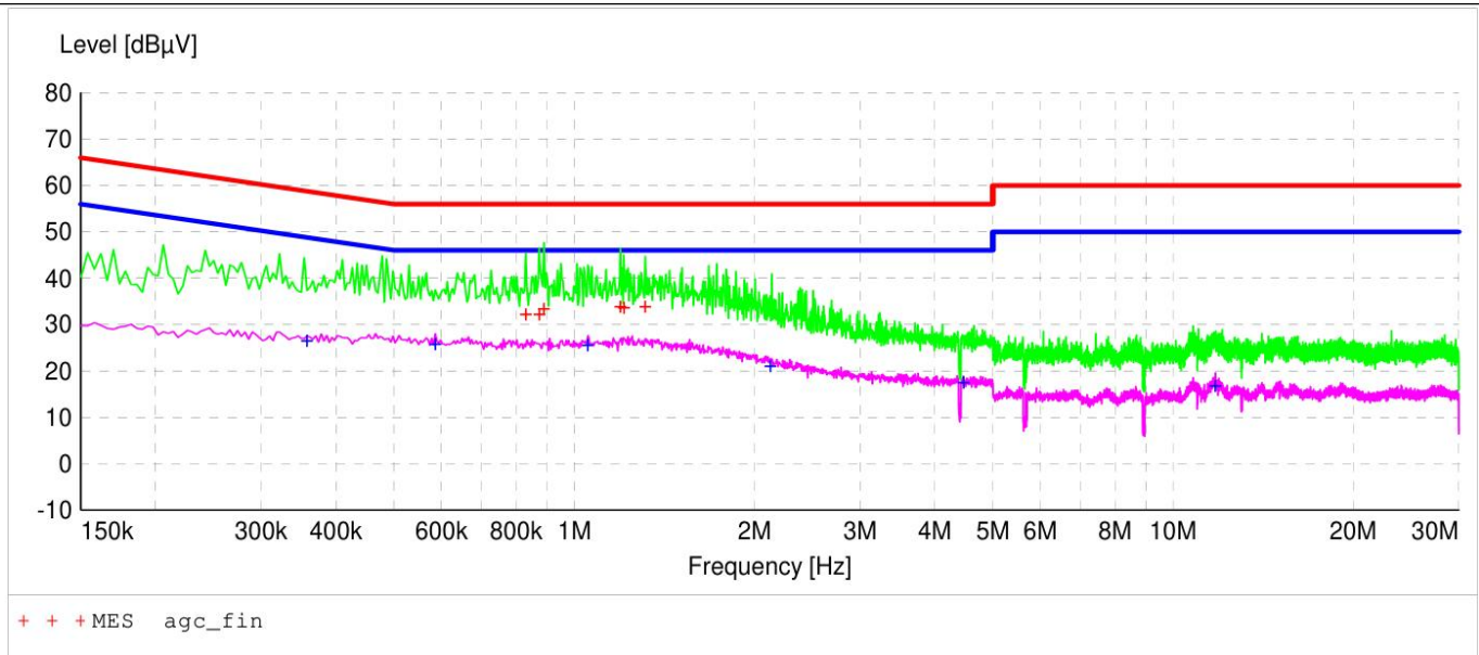
Test graph and data for Conducted Emission at line L1
