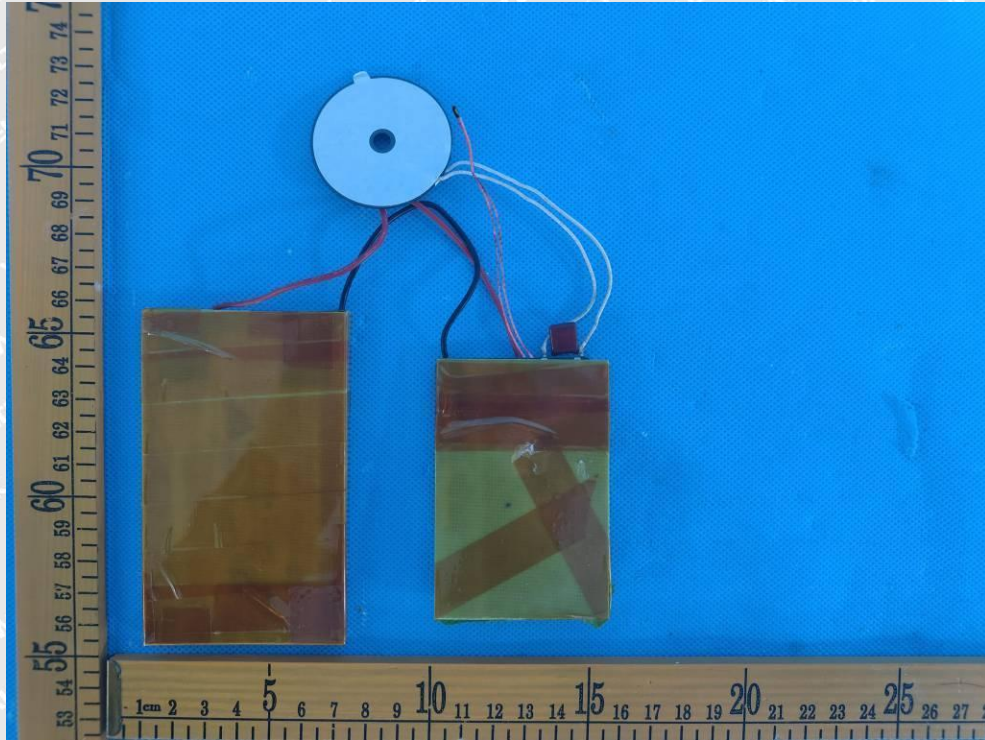
Photo 5: Internal view
