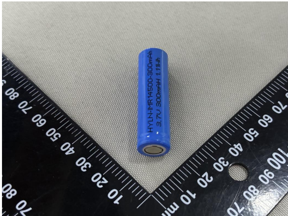
Figure 8 Side view of cell (IMR14500-300mAh)
