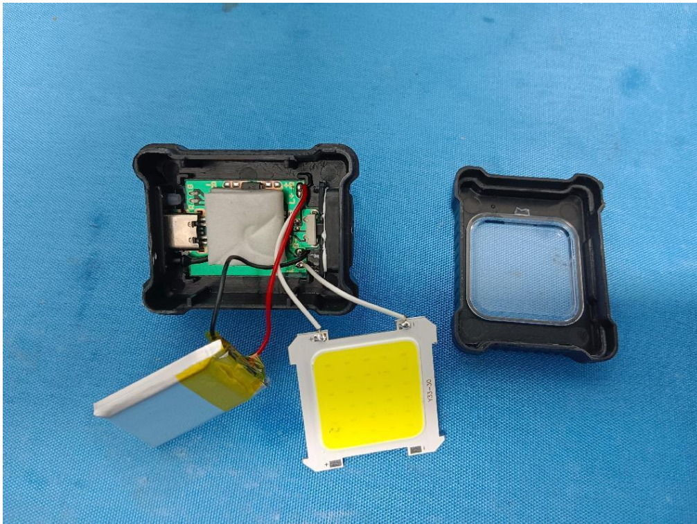
Fig.6 – Open view after IPX2 test
