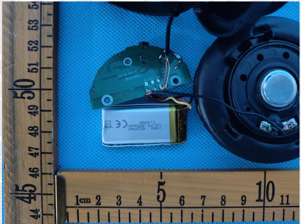
Figure 4: Internal view
