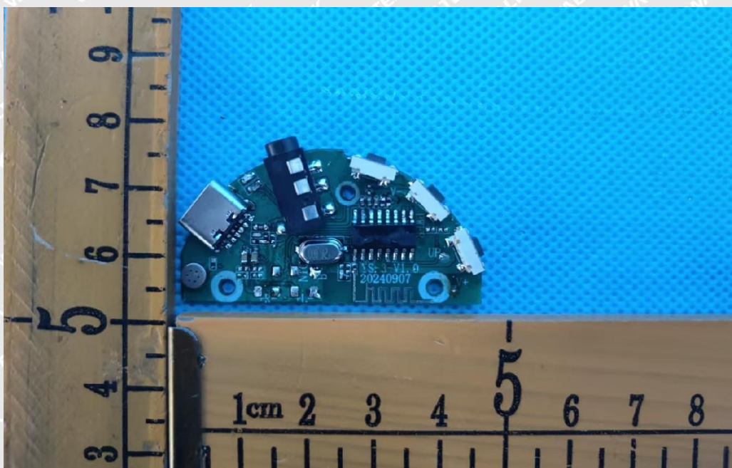
Figure 5: PCB view
