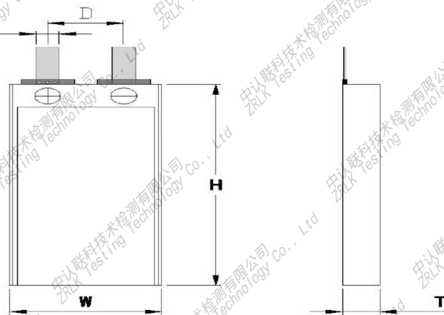
T*W*H=5.6 (max)*20.5 (max)*40.3 (max) Cell (Unit: mm)
