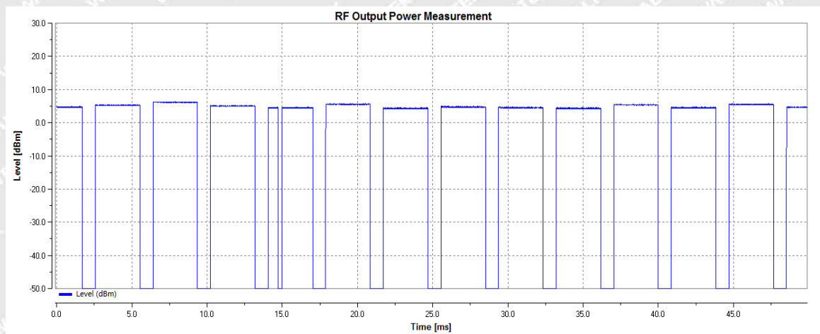
RF Output Power_THVN_DH5
