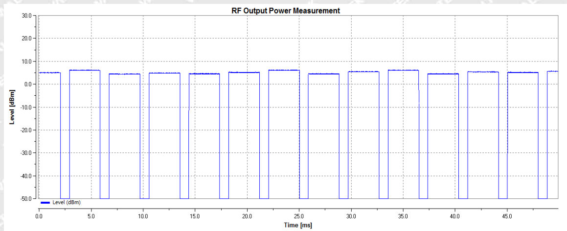
RF Output Power_TNVN_DH5
