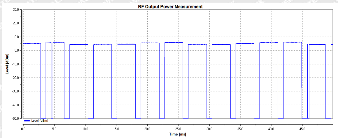
RF Output Power_TLVN_DH5
