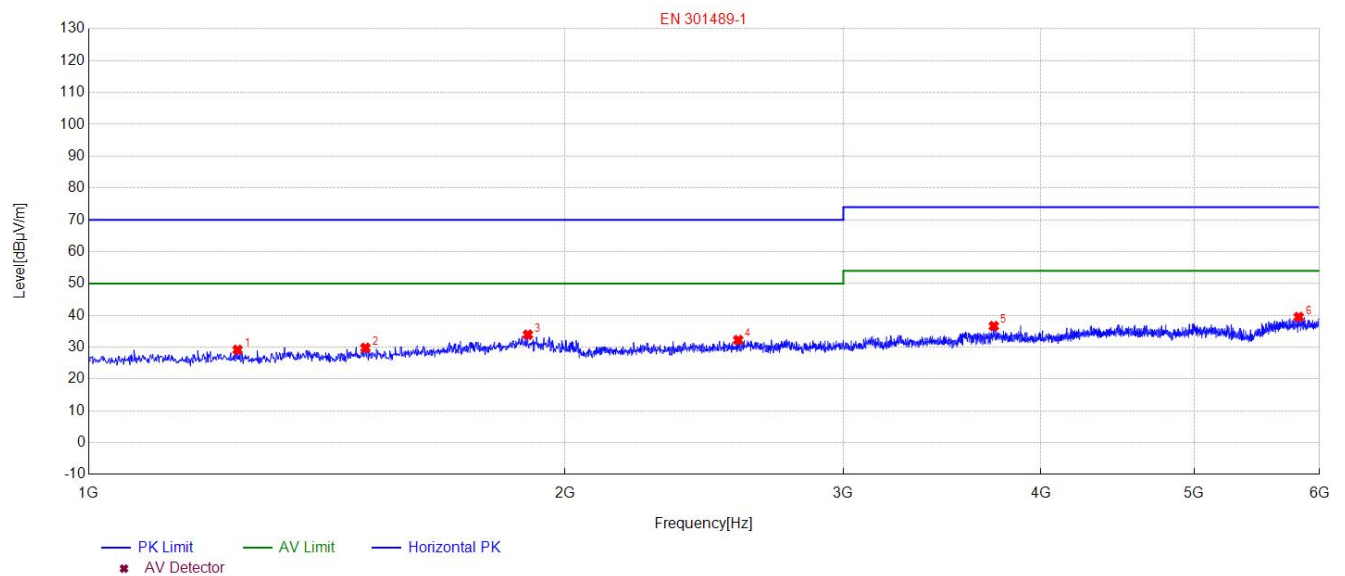
Test graph and data for Radiated Emission Above 1GHz at Horizontal
