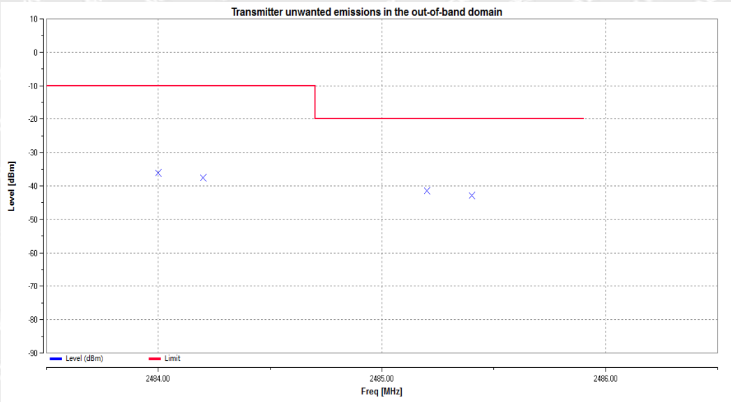
OOB_2DH5_Hop_2483.5MHz to 2483.5MHz+2BW
