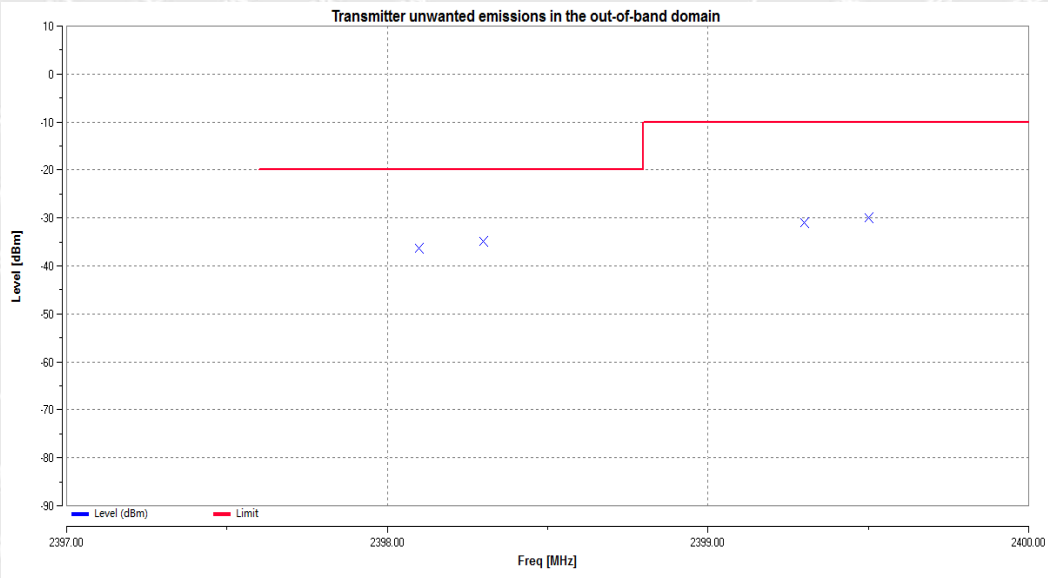
OOB_2DH5_Hop_2400MHz-2BW to 2400MHz
