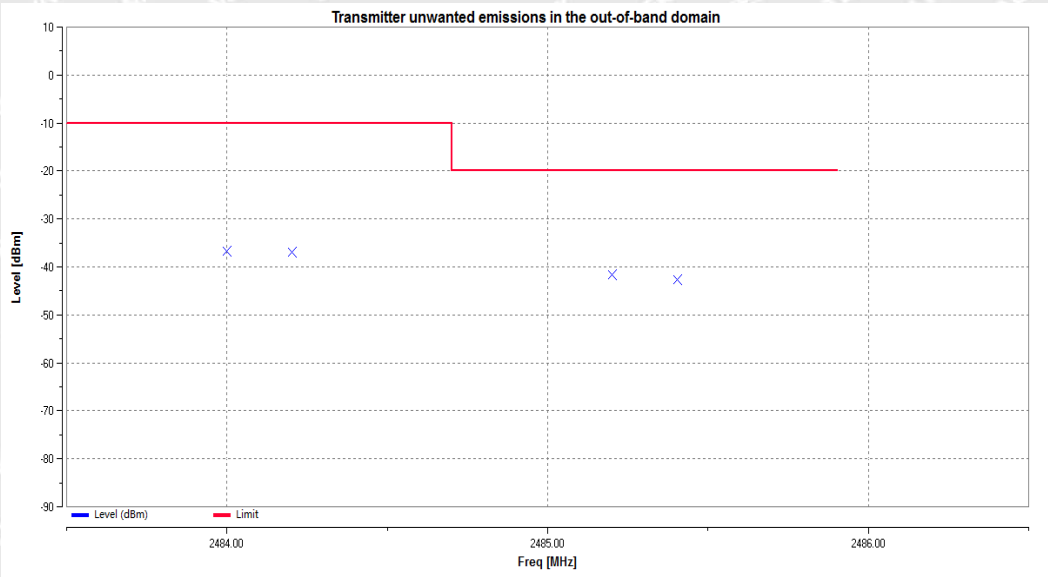
OOB_3DH5_Hop_2483.5MHz to 2483.5MHz+2BW
