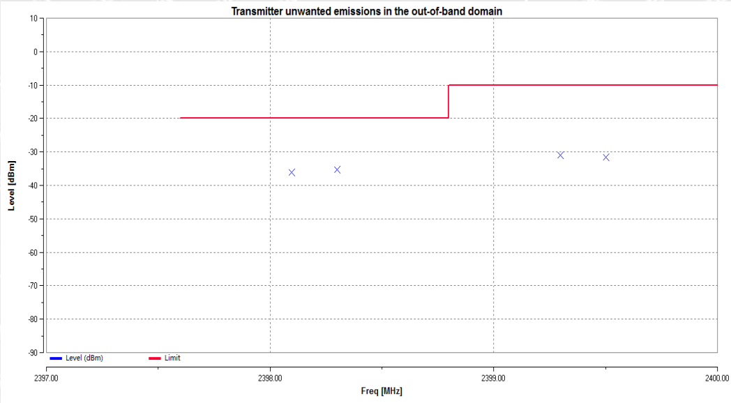
OOB_3DH5_Hop_2400MHz-2BW to 2400MHz
