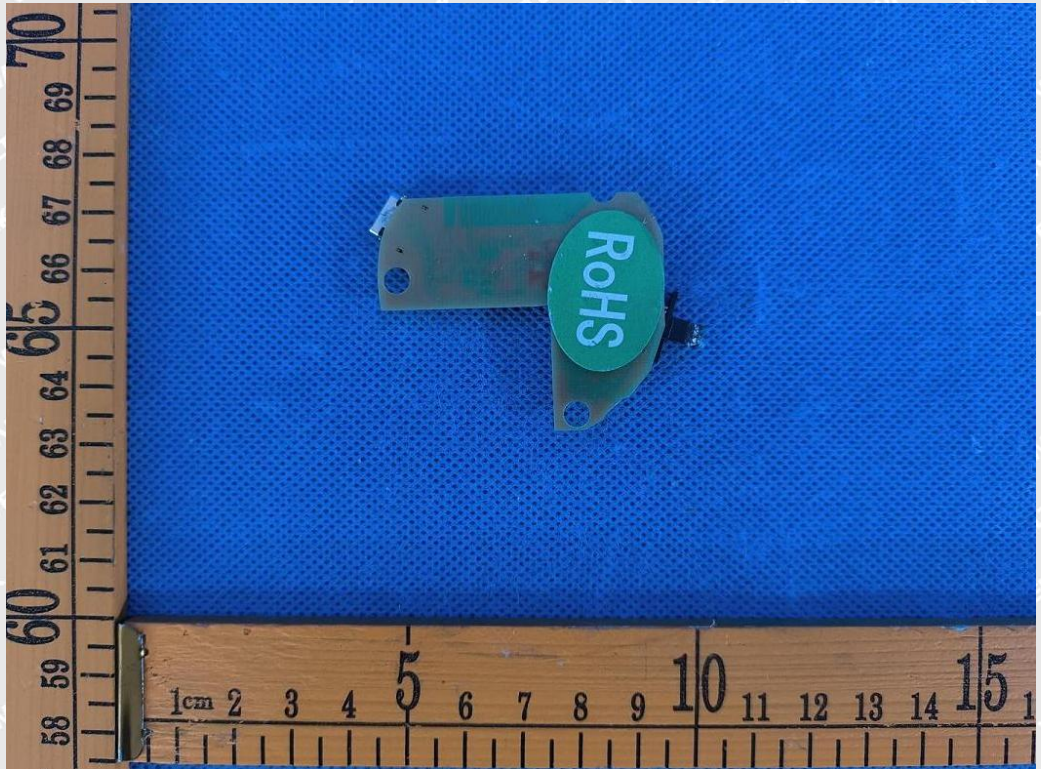
Figure 5: PCB view
