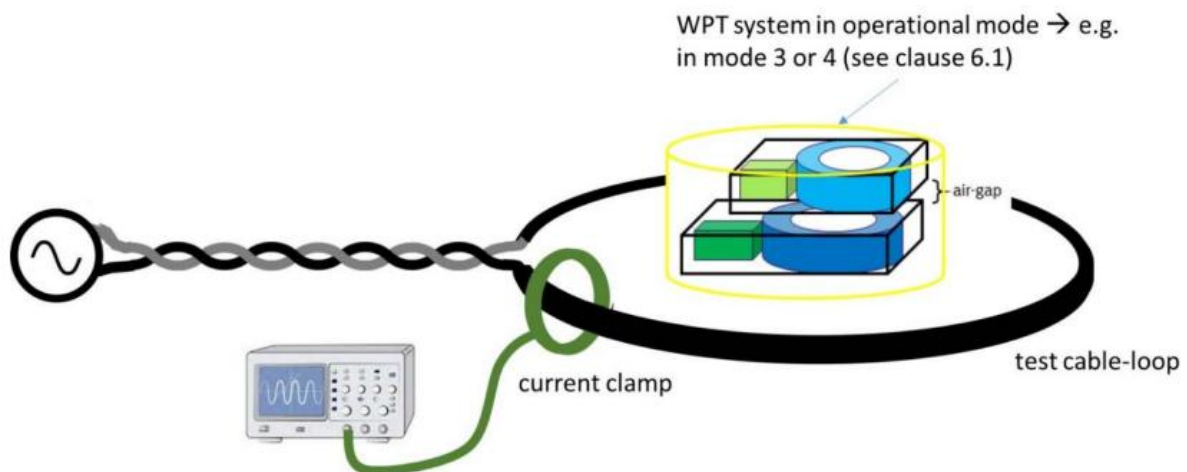
Figure 11: Schematic test set-up for the RX-blocking test
