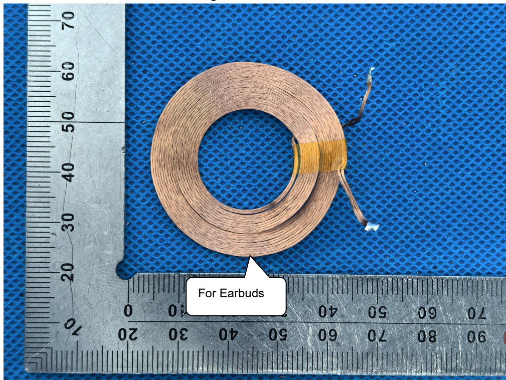
Fig. 12 – Coil view
