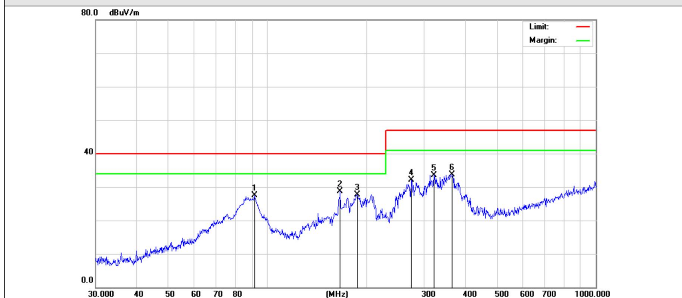
Test graph and data for Radiated Emission up to 1GHz
