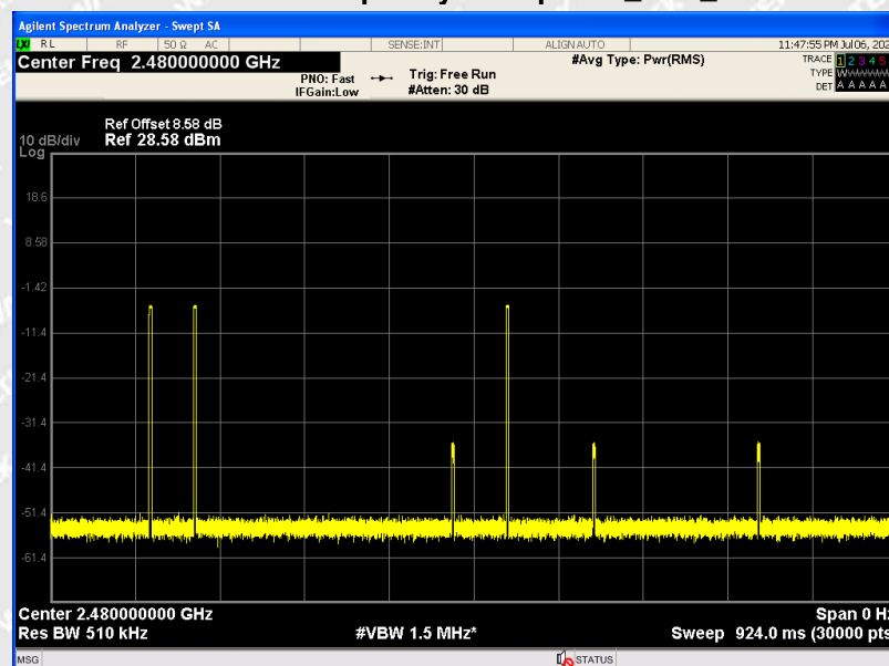
Minimum Frequency Occupation_DH5_2480
