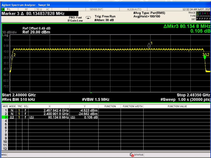
Hopping Sequence_2DH5
