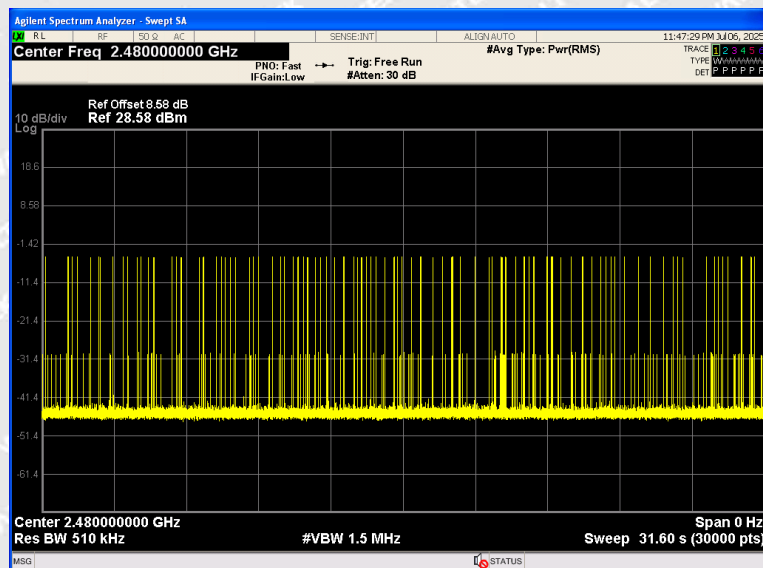
Accumulated Dwell Time_DH5_2480
