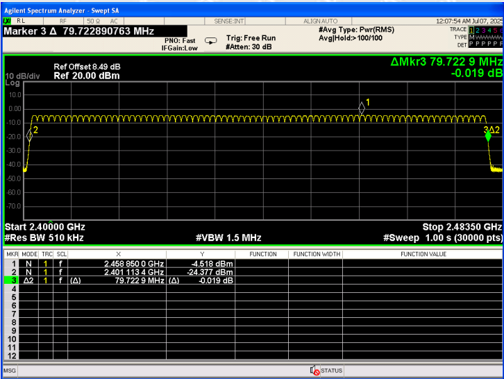
Hopping Sequence_DH5
