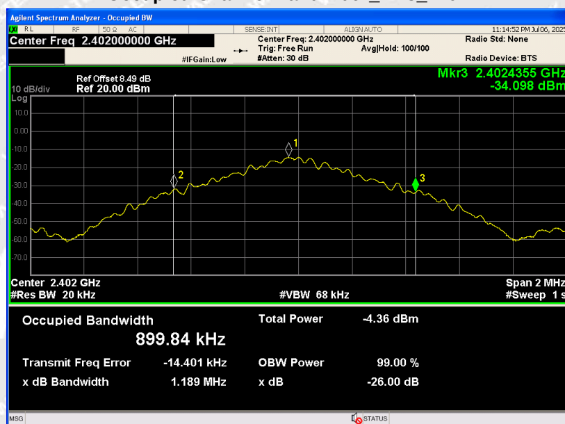
Occupied Channel Bandwidth_DH5_2402
