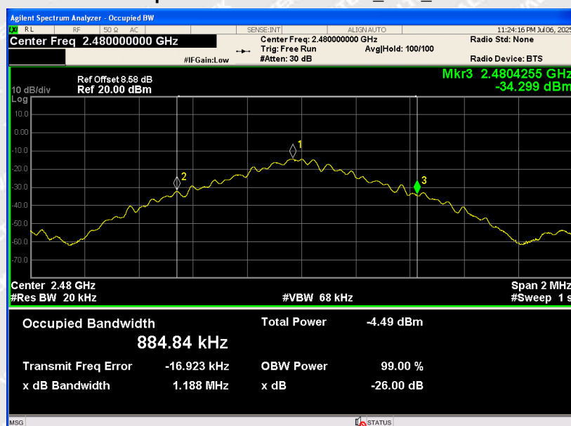
Occupied Channel Bandwidth_DH5_2480
