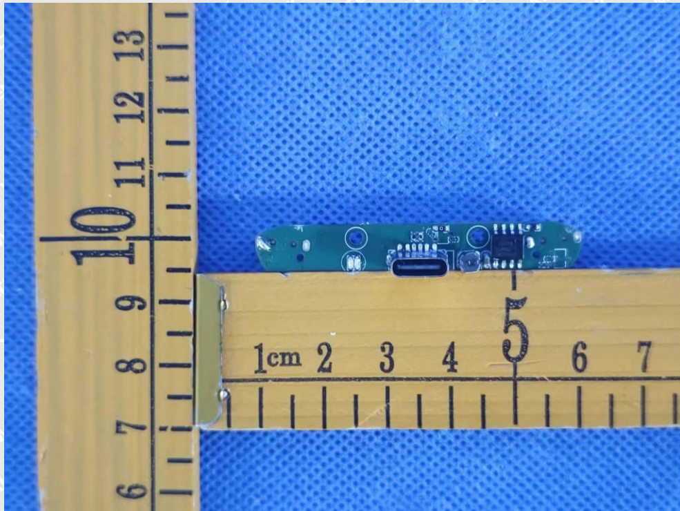
Figure 9: PCB view for charging base
