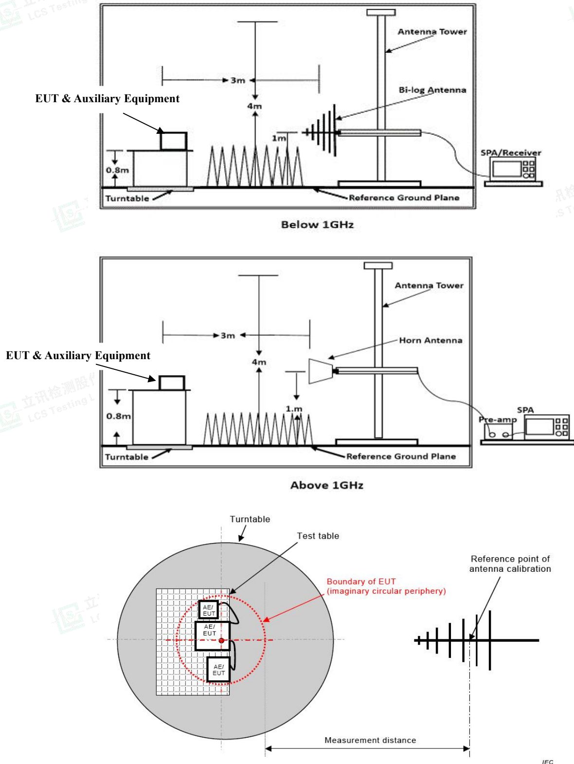
Figure C.1 – Measurement distance
